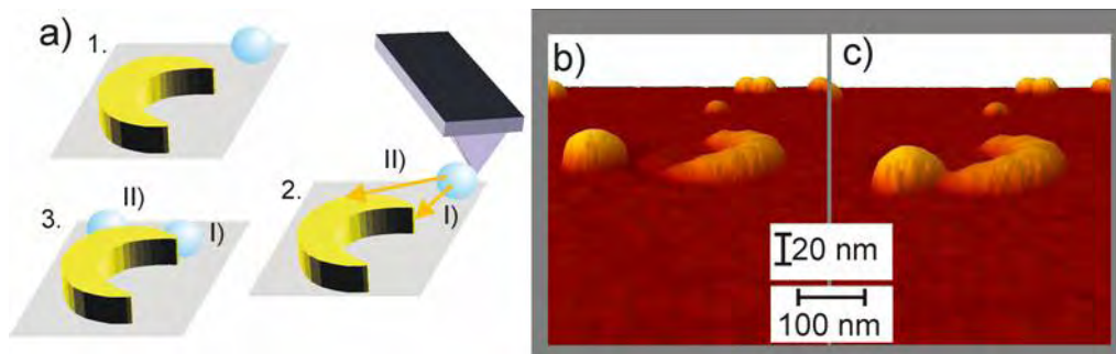
Fig. 2: a) Cartoon illustrating the attachment of a dielectric sphere to a gold crescent by AFM nanomanipulation. b,c) Crescent and Sphere before and after attachment as seen in the AFM.
