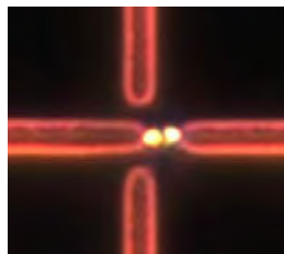
Fig. 2: Conductive bridge made from 30nm gold nanoparticle ( R < 1000\Omega )
