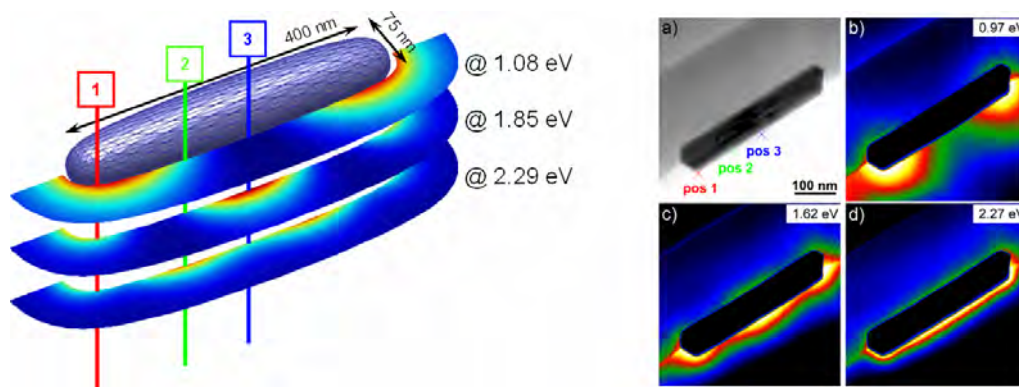
Figure 1: Results of a boundary element method simulation (left panel) and experiment (right panel). Triangulated surface of rod-shaped nanoparticle and EFTEM maps as computed and measured according to the prescription of Ref. [2].
