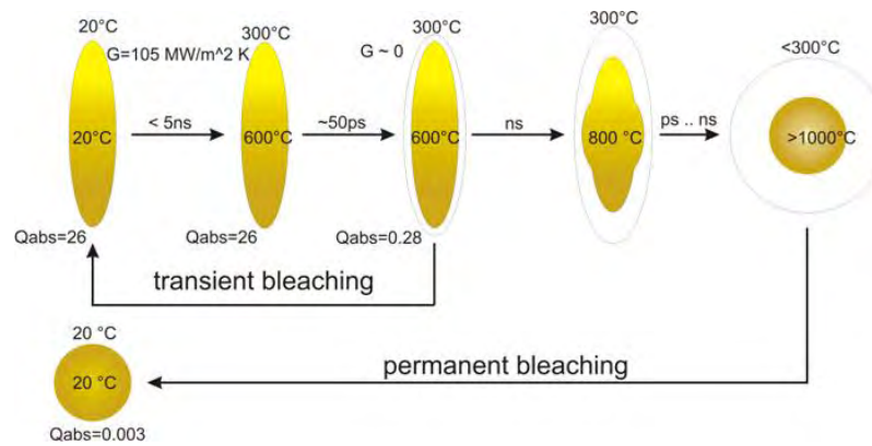
Figure 1: Model for the temperature increase, absorption and particle shape change during the nanosecond pulsed irradiation
