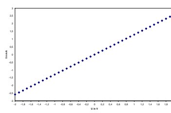
Fig. 3: V-I characteristic of 30 nm gold nanoparticle bridge
