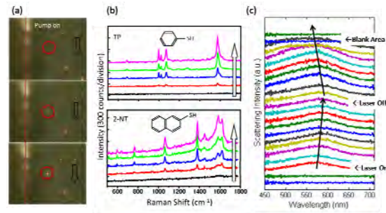
Figure 2: (a), (b) Dark-field (DF) images and temporal SERS spectra recorded during a trapping process in a microfluidic channel. (c) DF scattering spectra measured during trapping between two glass slides.
