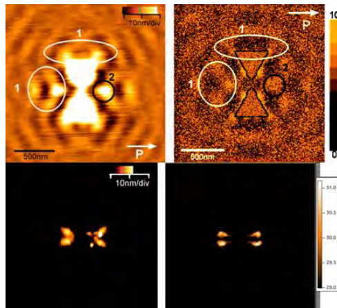
Figure 1. Images of the sample surface after irradiation. The polarization is perpendicular to the major axis of the bowtie. (a) and (c) were obtained by AFM and (b) and (d) are the corresponding calculations.
