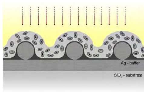
Schematization of the system with on a nanocrystals distribution for a Metal-Enhanced Fluorescence application.
