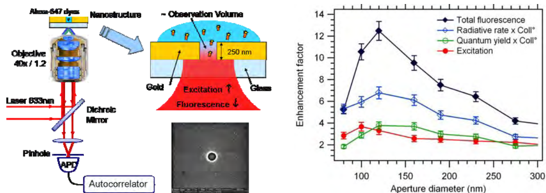
Fig. 1: (Left) Schematic view of the experimental setup: the emission from dyes diffusing in a nanoaperture is detected through a confocal microscope in epi-fluorescence configuration. (Right) Physical contributions to nanoaperture enhanced fluorescence, plotted versus the aperture diameter and normalized to the open solution case.
