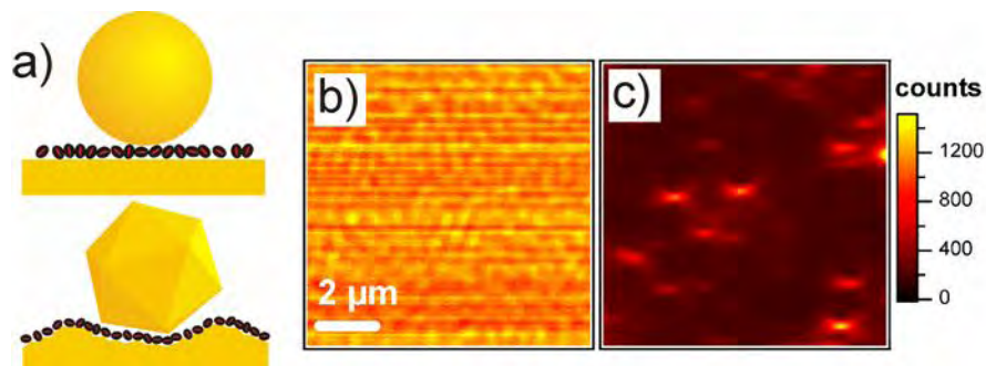
Fig. 1: a) Sketch of an ideal sphere-on-plane geometry as assumed for modelling (left) in comparison to a realistic sketch, taking into account crystallinity of the metal colloid and the typical roughness of a metal film (right). b) Colloid-decorated gold surface seen with standard (left) and plasmon mediated dark field microscopy (right)
