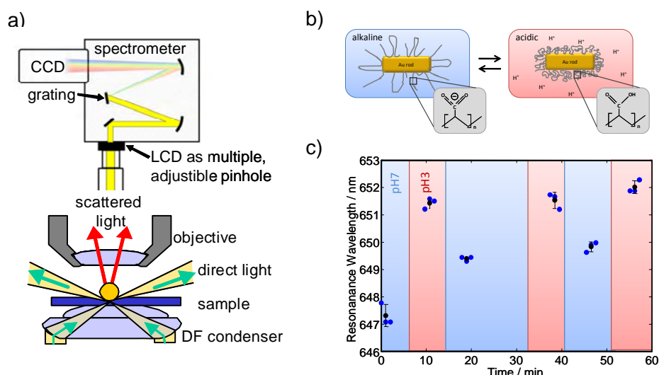
Figure 1a) Schematic view of the darkfield microscope. b) Scheme of the developed pH-sensor. pH is triggering the packing density sensed by the Plasmon. c) Shifting resonance position of one single particle in changing pH conditions.
