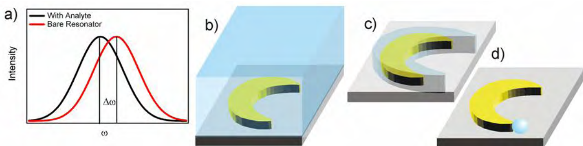
Fig. 1: a) sketch for a resonance shift. b) Crescent-shaped resonator immersed in bulk dielectric. c) coating with a layer. d) Attachment of a dielectric sphere.
