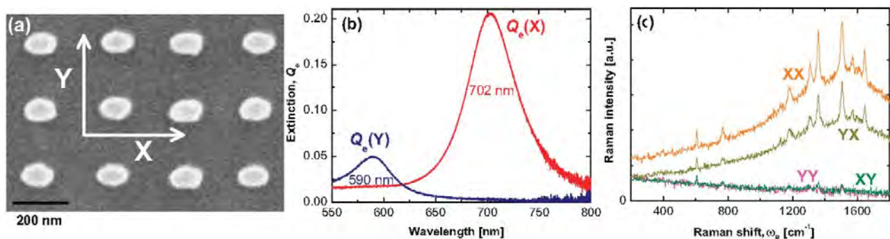
Fig. 1: (a) SEM image of an array of prolate gold nanoparticles. (b) Extinction spectrum of the array for X- and Y-polarization. (c) SERS spectra for the four excitation-detection polarization configurations.
