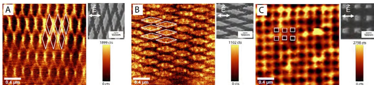
Figure 2. Scanning near-field optical microscopy (SNOM) image of the nanorhombs (A) and (B) and nanosquare (C) surfaces. SNOM experiments in the pick-up mode were performed with laser excitation at 633 nm. Therefore the plasmonic array is illuminated with linear polarized laser light from below and the transmitted light is collected through a small aperture (~150 nm). With the E-field of the incident light being parallel to the short axis of the nanorhombs (A) local field enhancement in the gap between individual nanoparticles is observed. (B) By rotating the plasmonic array by 90 degree, i.e. the E field being parallel to the long axis, only a reduced field enhancement due to the intrinsic roughness of the gold film is detected. (C) SNOM image of the nanosquares.
