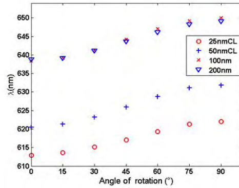
LSPR shift as a function of director's orientation.
