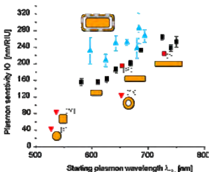
Figure Overview of the sensitivity \mathcal{S} = d\lambda_{\text{res}} / dn of different gold nanostructures: spheres, cubes, rods, shells, and rod-shaped nanorattles. Since the sensitivity depends not only on shape but also on the position of the resonance wavelength, we show the sensitivity values as a function of the plasmon wavelength in water. The values for spheres, cubes, shells, and some rod samples are taken from the literature. Our data for ensemble measurements on different samples of solid gold nanorods (black labels) show lower \mathcal{S} values than rod-shaped gold nanorattles, produced from these rods (blue labels).
