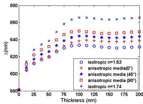
LSPR shift for several LCM thicknesses.
